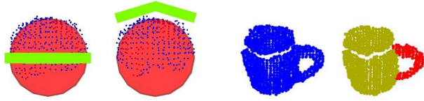
Fig. 4. Left: Grasp Generation for Spherical Objects. Detected grasps (green) for spherical object point cloud data (blue) and the best fit 3D shape primitive (red). Right: Clusters of points on the cylindrical shape surface (yellow) are marked as protrusions (red).
